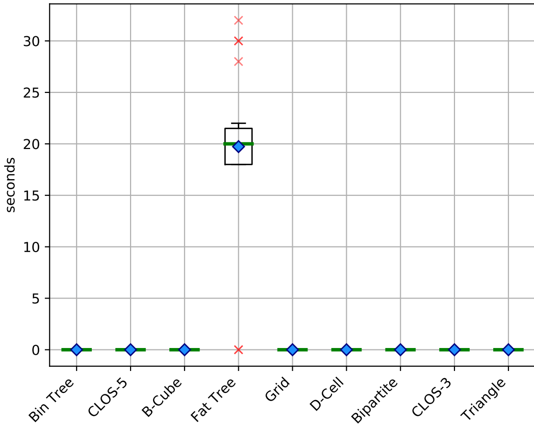
Routing response time using LDR (single-path)
