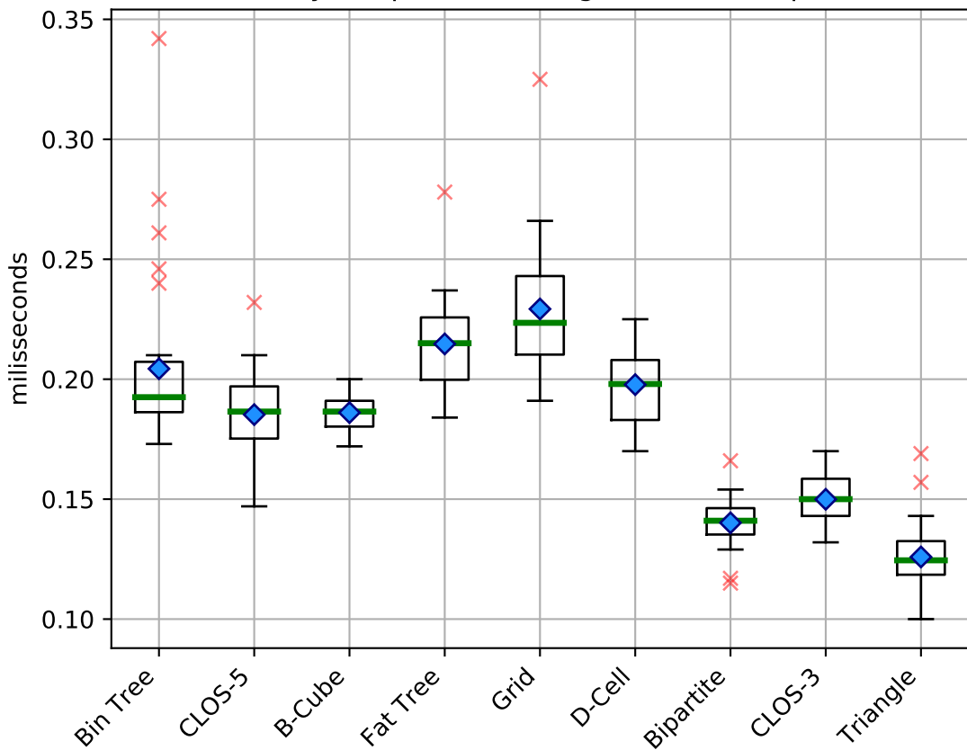
Latency (sequential) using ECMP (multi-path)
