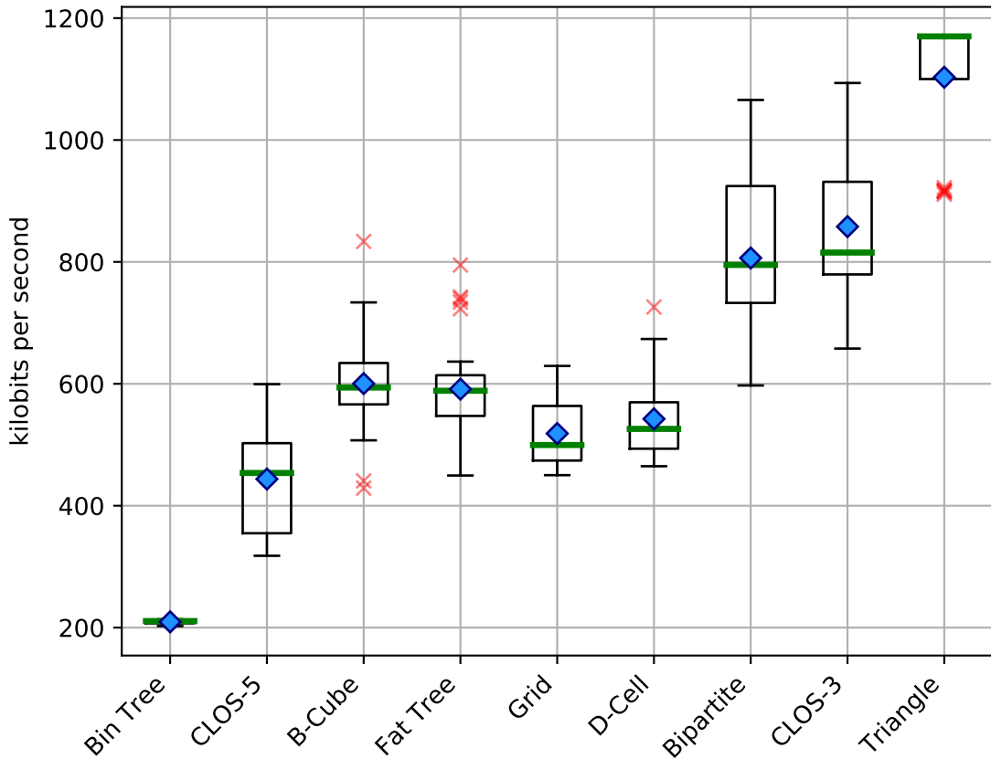
Bandwidth (concurrent) using ECMP (multi-path)
