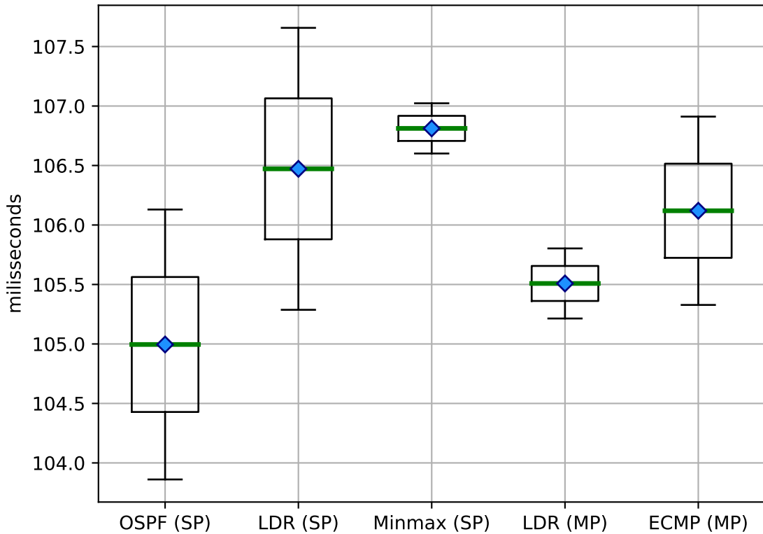
Jitter (impact) on Binary Tree
