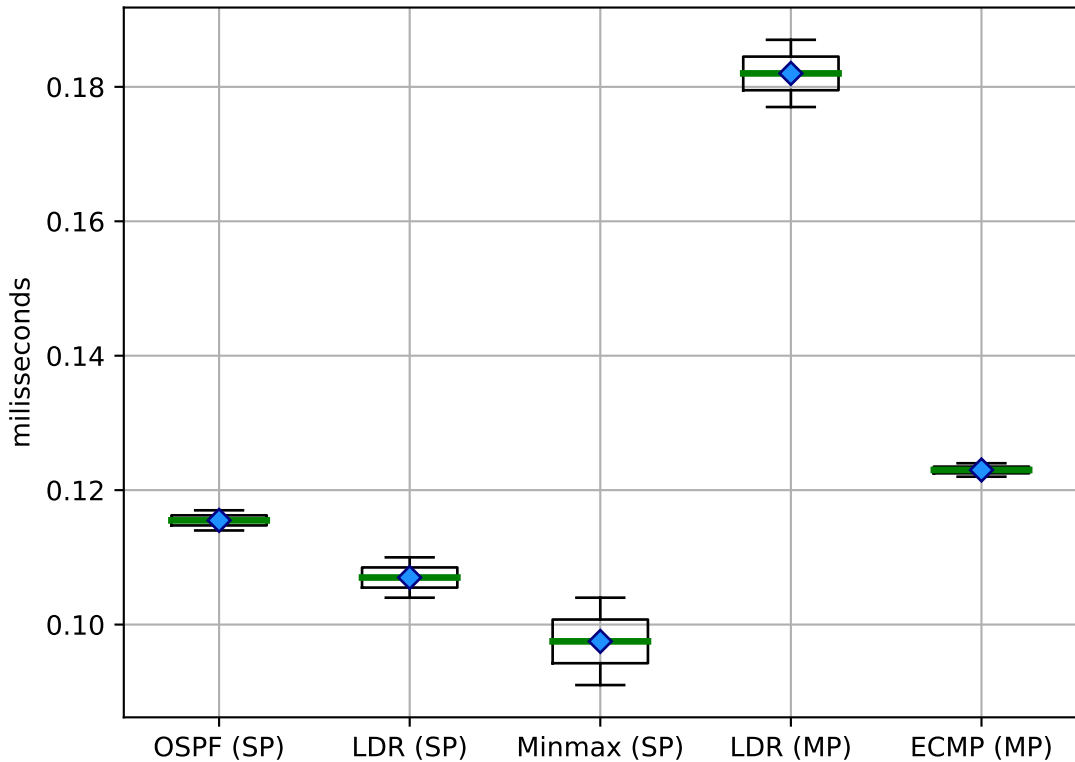
Latency (sequential) on Triangle
