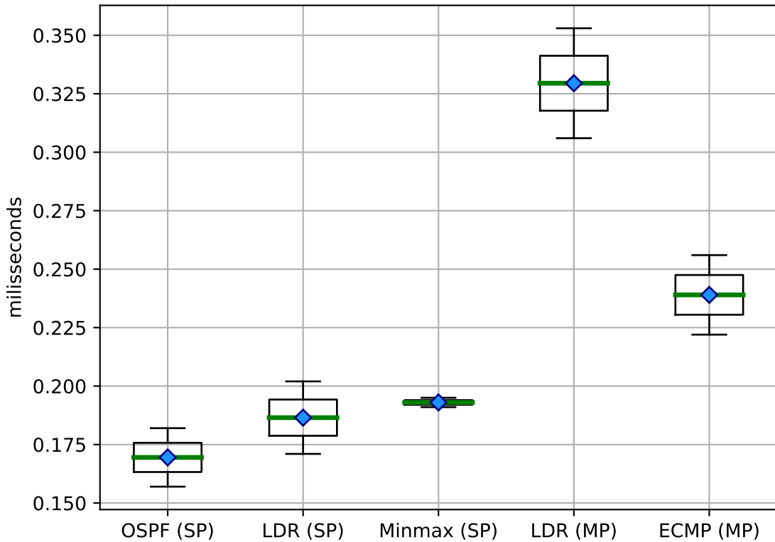
Latency (sequential) on Grid
