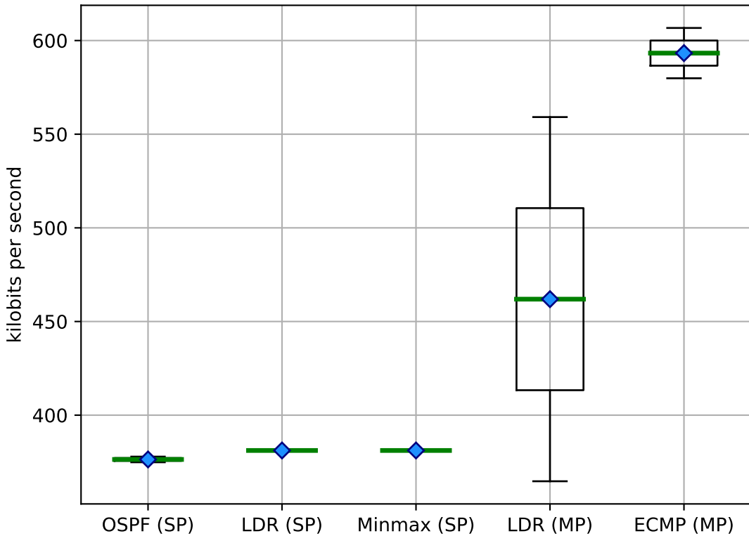
Bandwidth (concurrent) on Fat Tree
