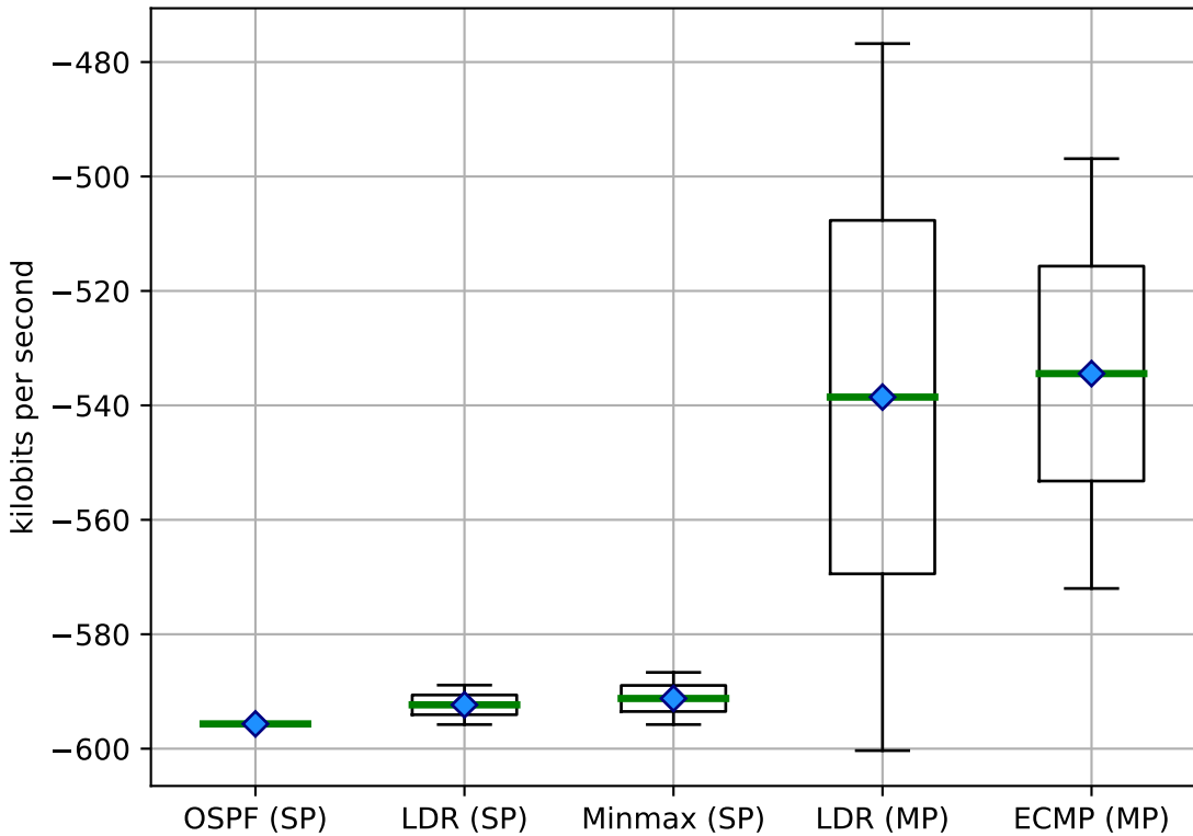
Bandwidth (impact) on D-Cell
