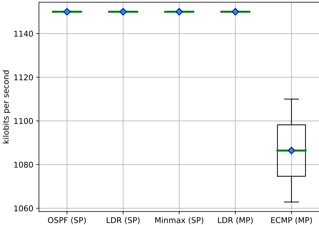
Bandwidth (sequential) on 5-layered CLOS
