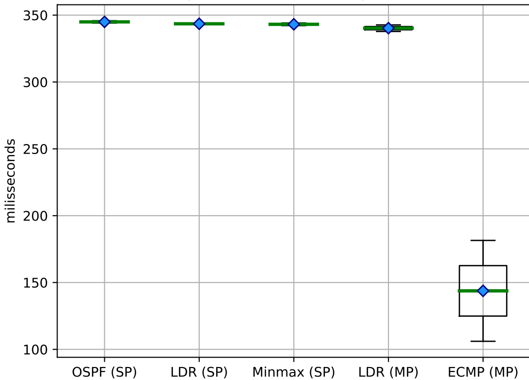
Latency (concurrent) on 5-layered CLOS
