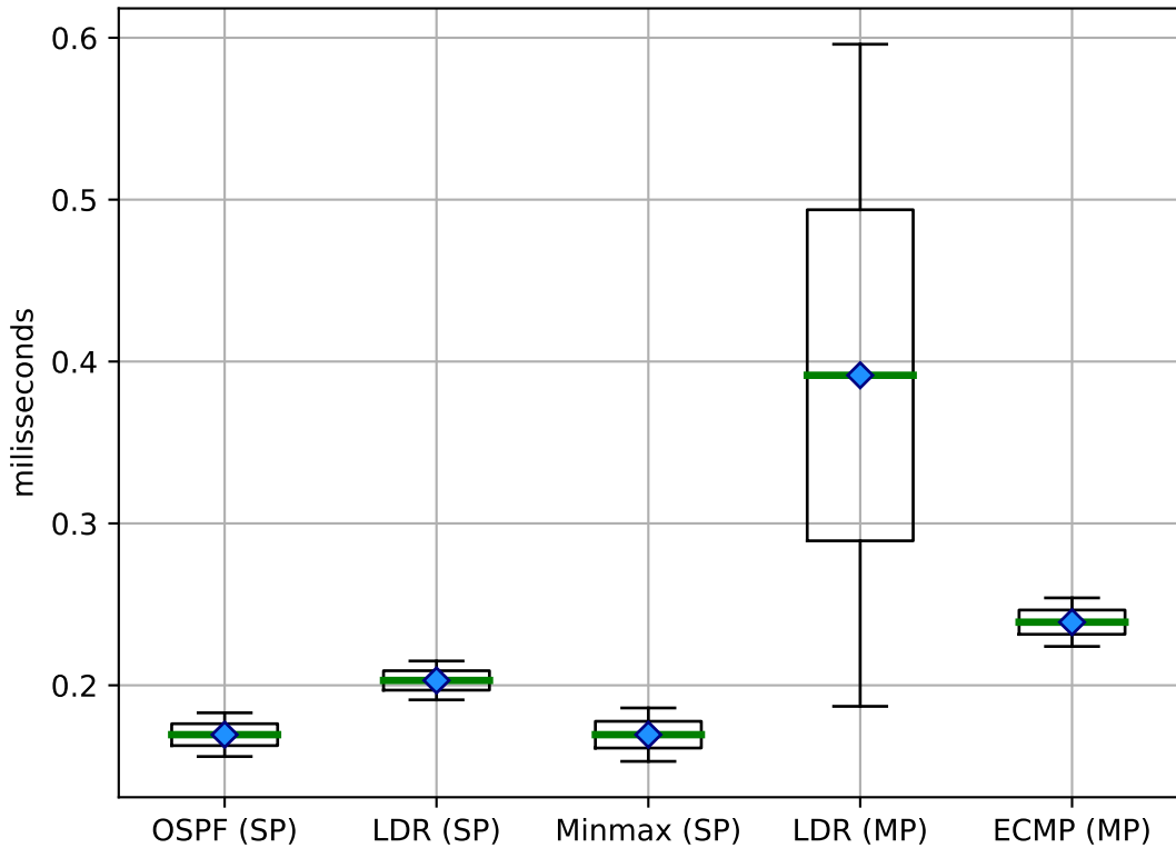
Jitter (sequential) on 3-layered CLOS
