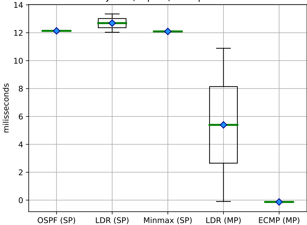
Jitter (impact) on Bipartite
