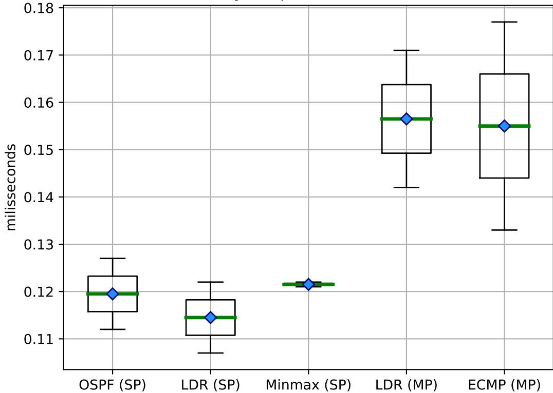
Latency (sequential) on B-Cube
