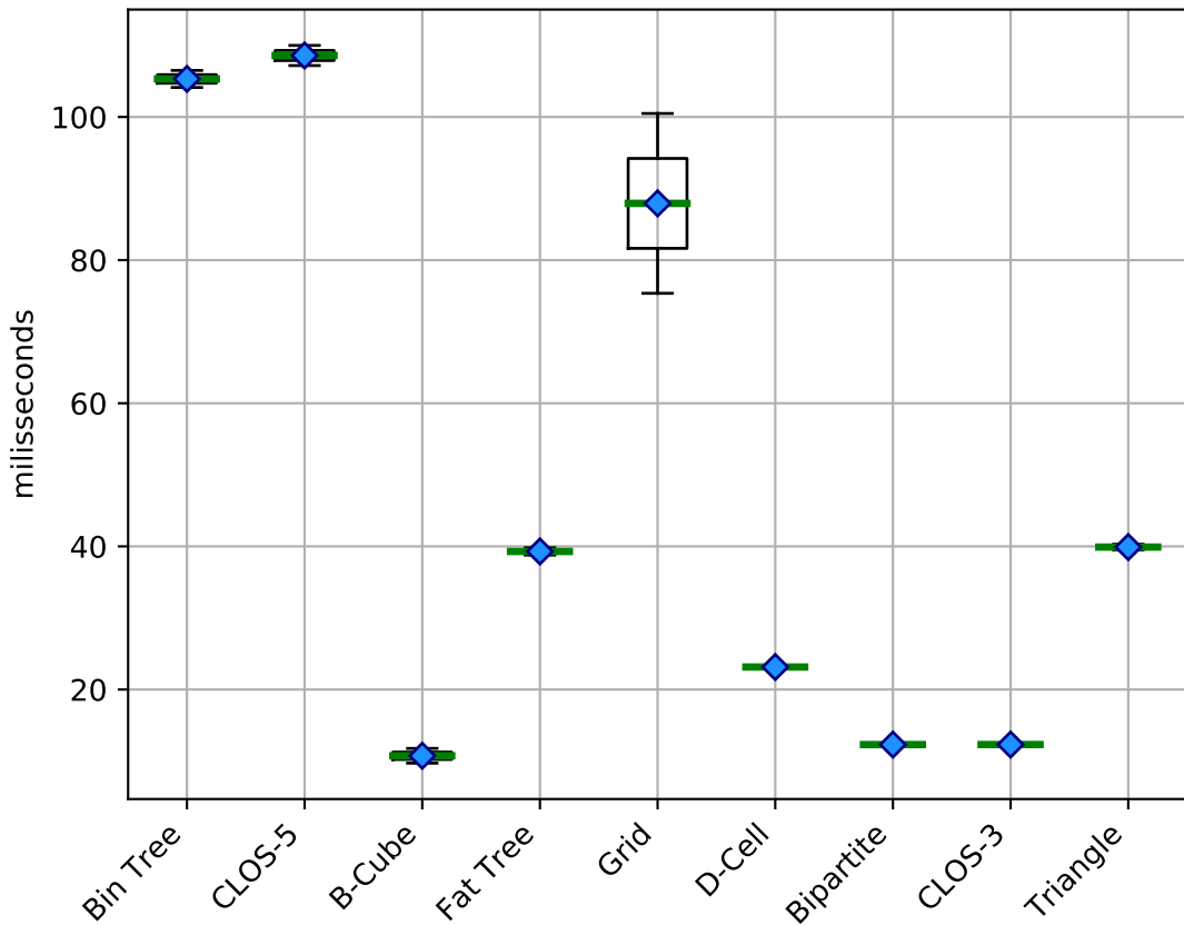
Jitter (concurrent) using OSPF (single-path)
