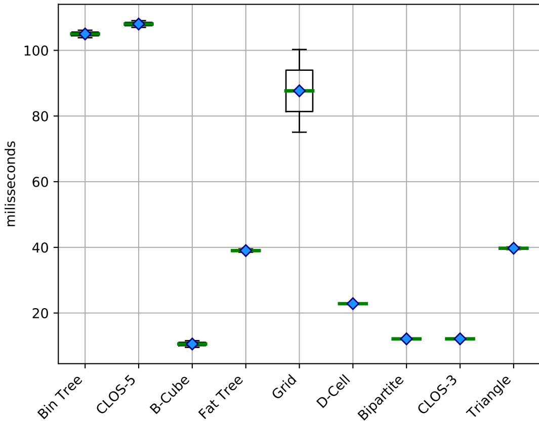
Jitter (impact) using OSPF (single-path)
