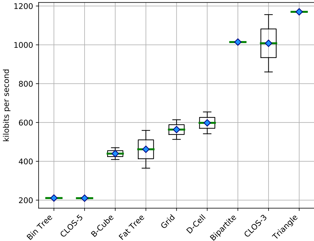
Bandwidth (concurrent) using LDR (multi-path)
