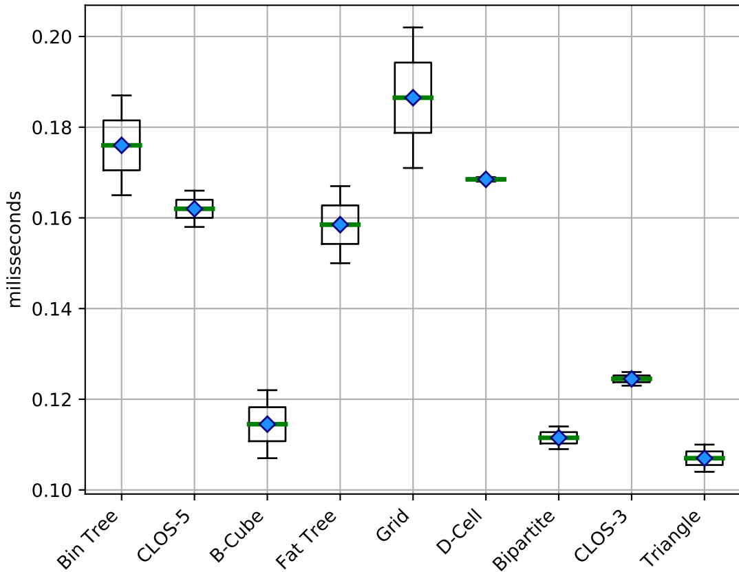
Latency (sequential) using LDR (single-path)
