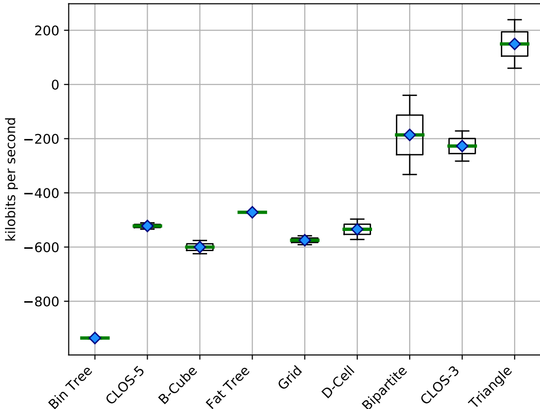
Bandwidth (impact) using ECMP (multi-path)
