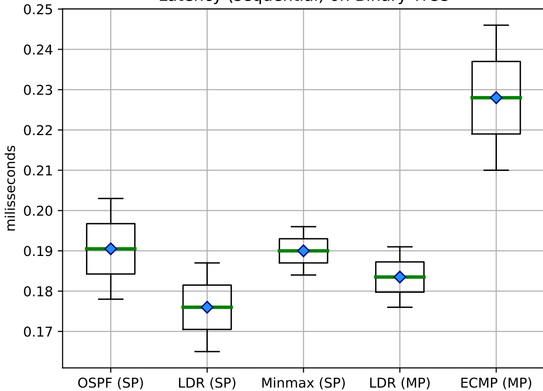
Latency (sequential) on Binary Tree
