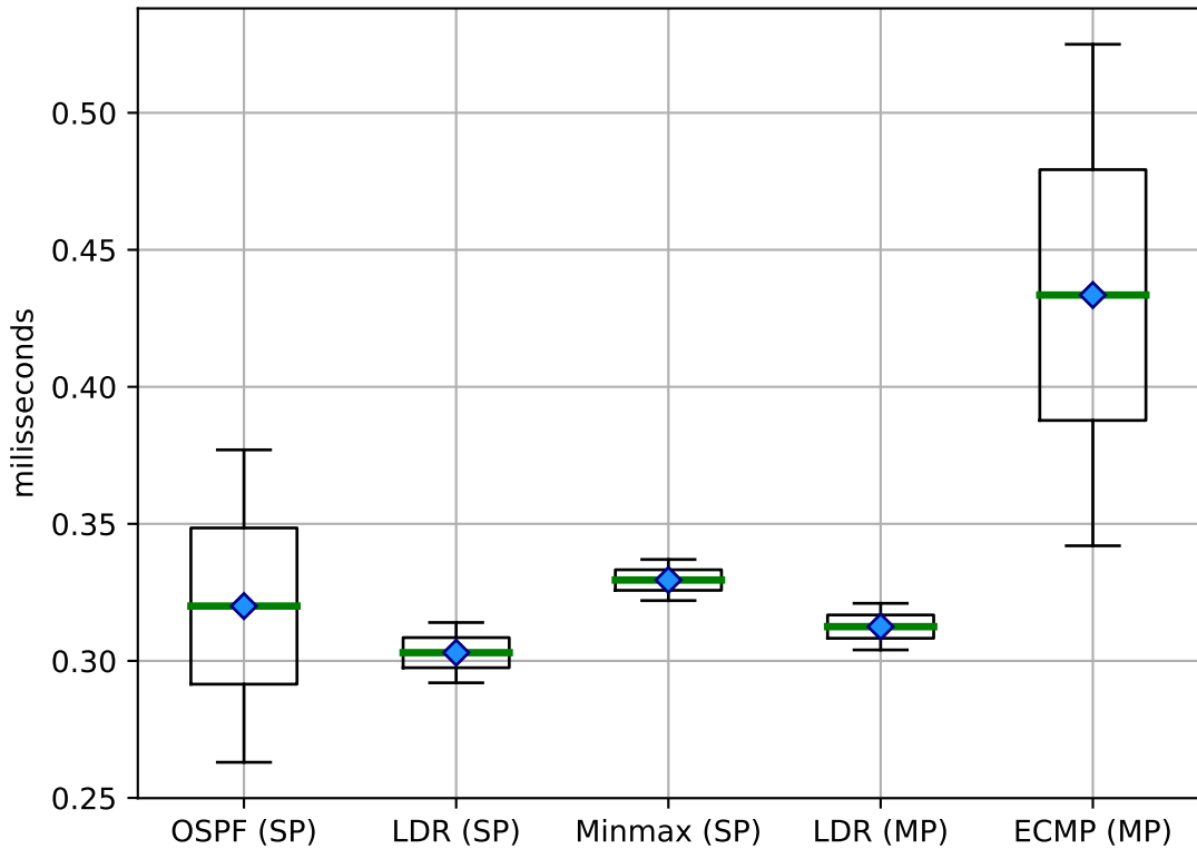
Jitter (sequential) on Binary Tree
