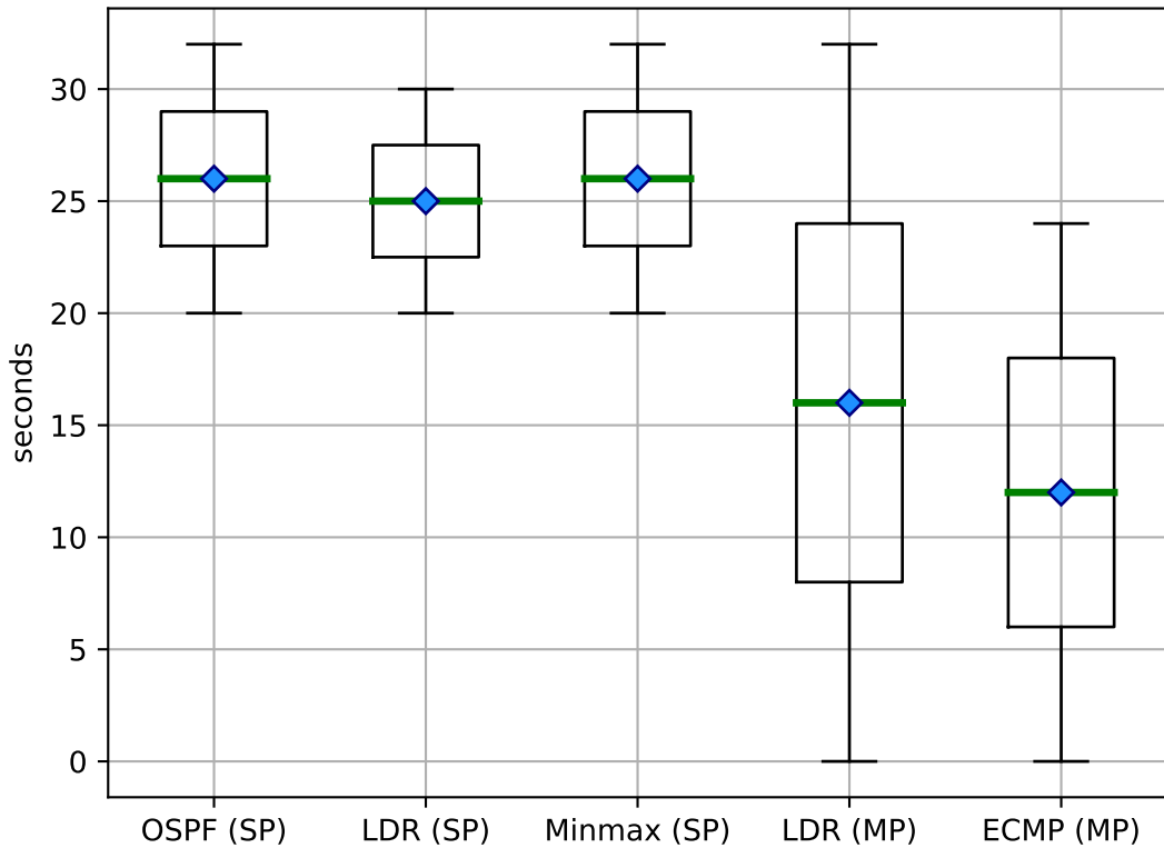
Routing response time on Fat Tree
