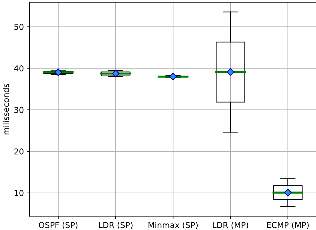
Jitter (impact) on Fat Tree
