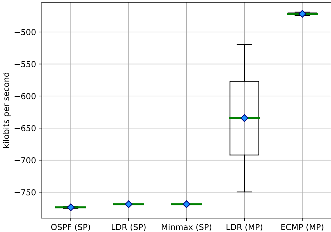
Bandwidth (impact) on Fat Tree
