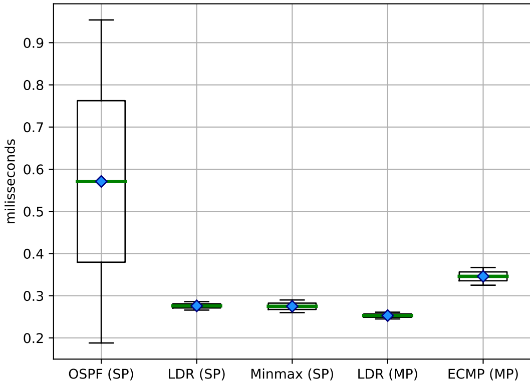
Jitter (sequential) on 5-layered CLOS
