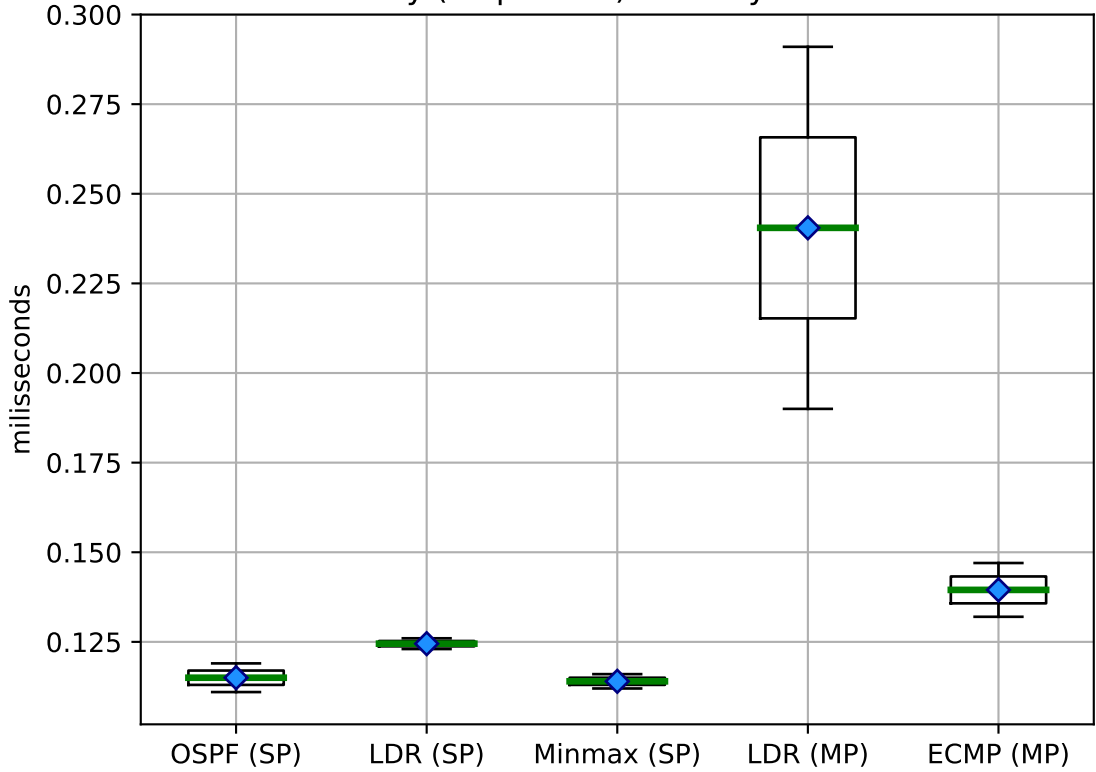
Latency (sequential) on 3-layered CLOS
