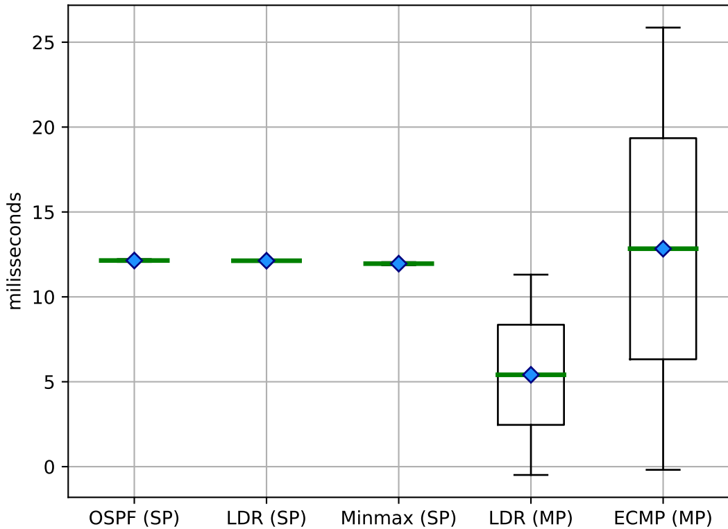
Jitter (impact) on 3-layered CLOS
