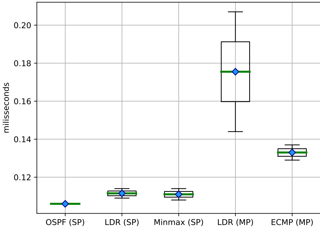
Latency (sequential) on Bipartite
