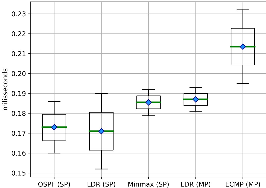
Jitter (sequential) on Bipartite
