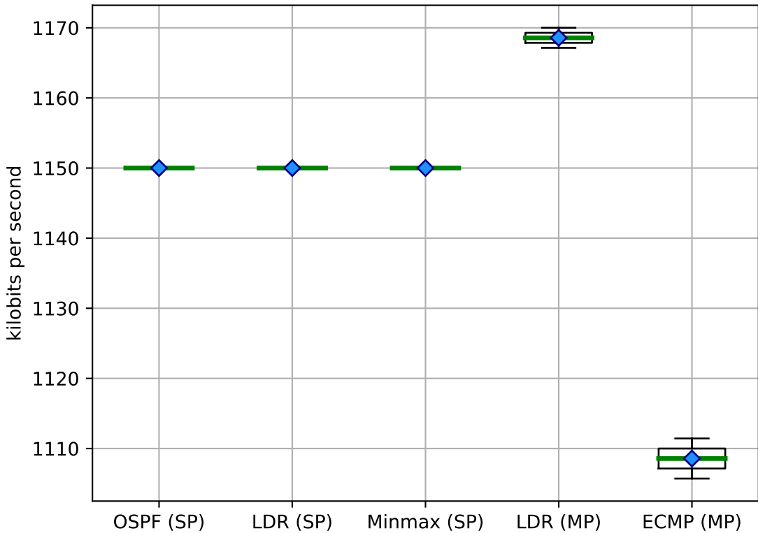
Bandwidth (sequential) on Bipartite
