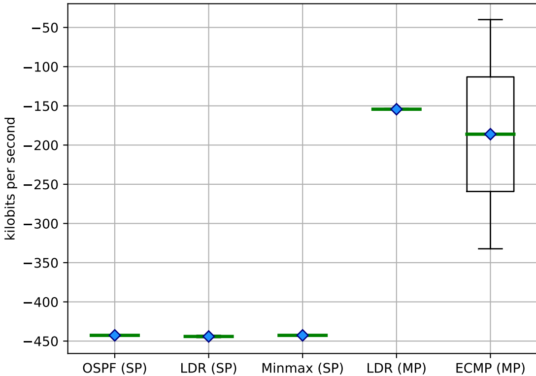
Bandwidth (impact) on Bipartite
