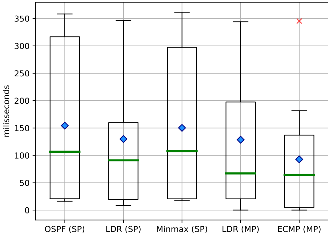
Latency (concurrent) on All
