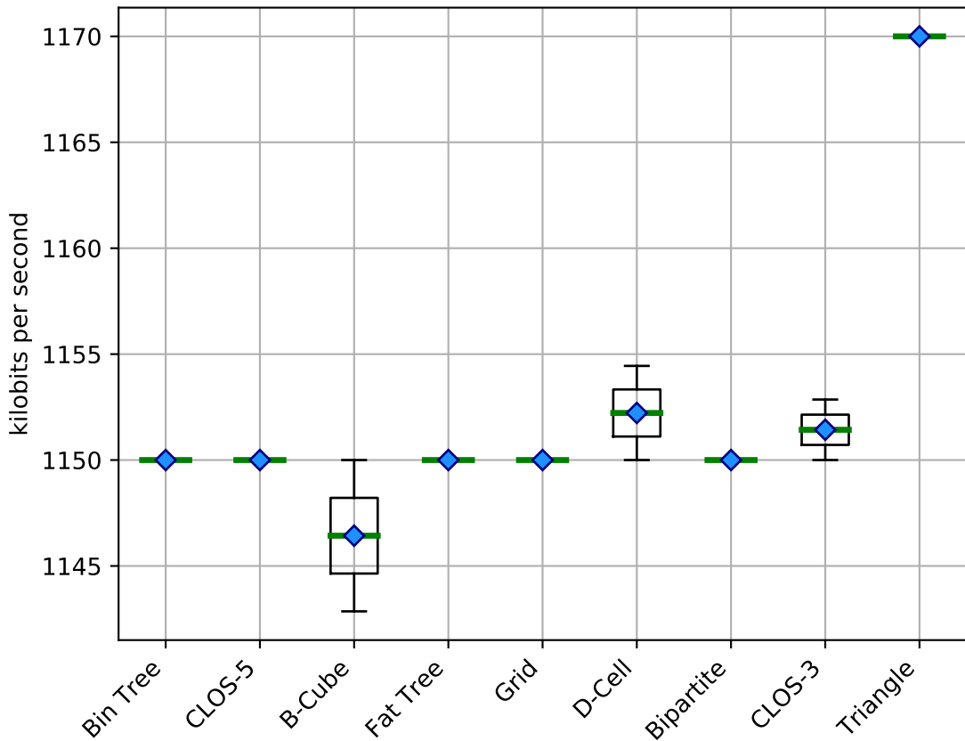
Bandwidth (sequential) using OSPF (single-path)
