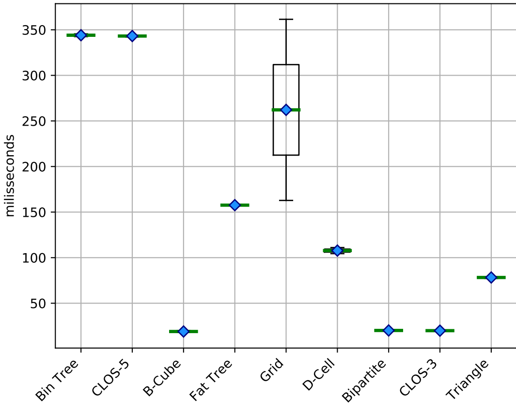
Latency (concurrent) using Minmax (single-path)
