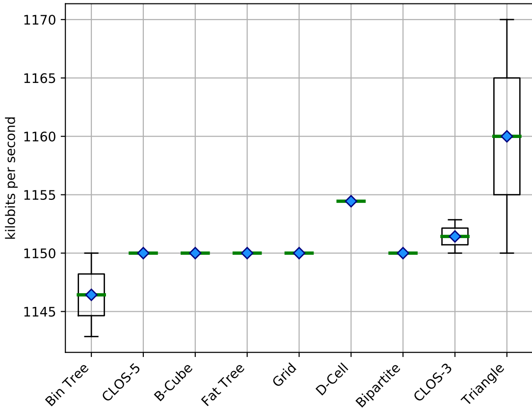
Bandwidth (sequential) using LDR (single-path)
