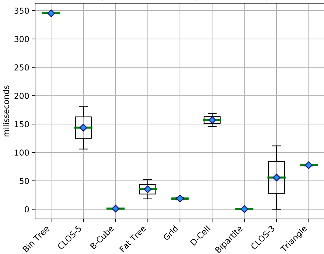
Latency (concurrent) using ECMP (multi-path)
