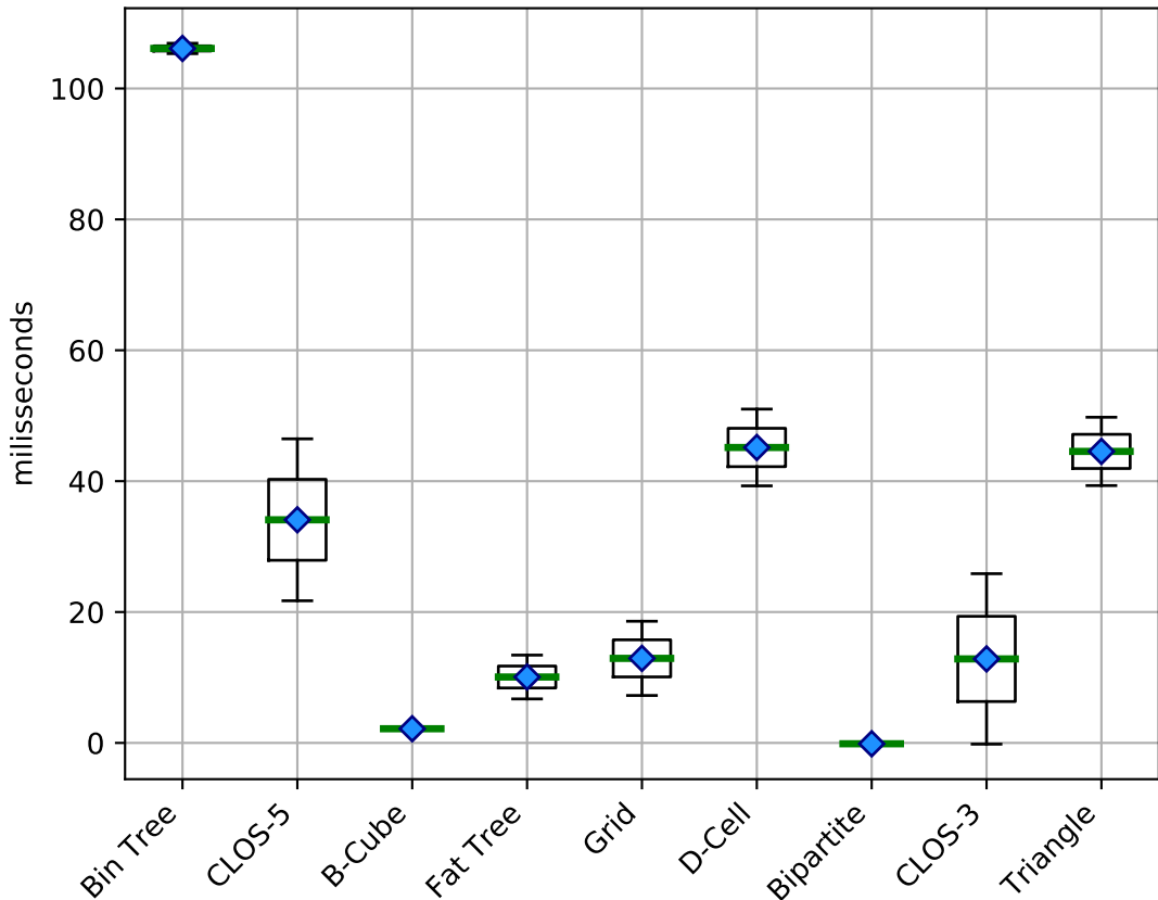
Jitter (impact) using ECMP (multi-path)
