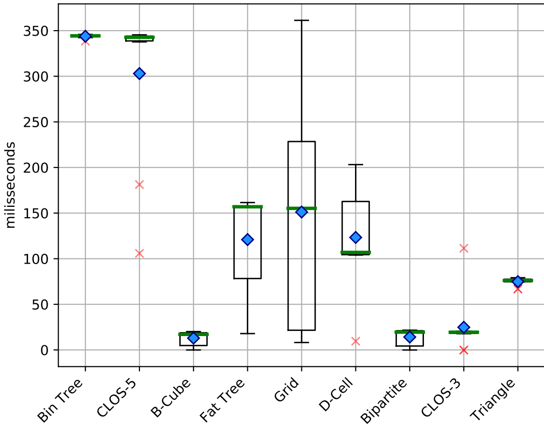
Latency (impact) using All
