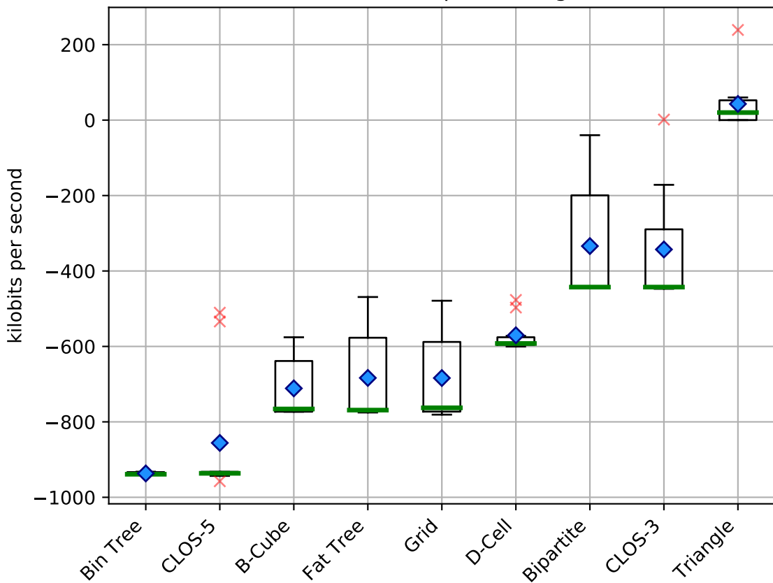
Bandwidth (impact) using All
